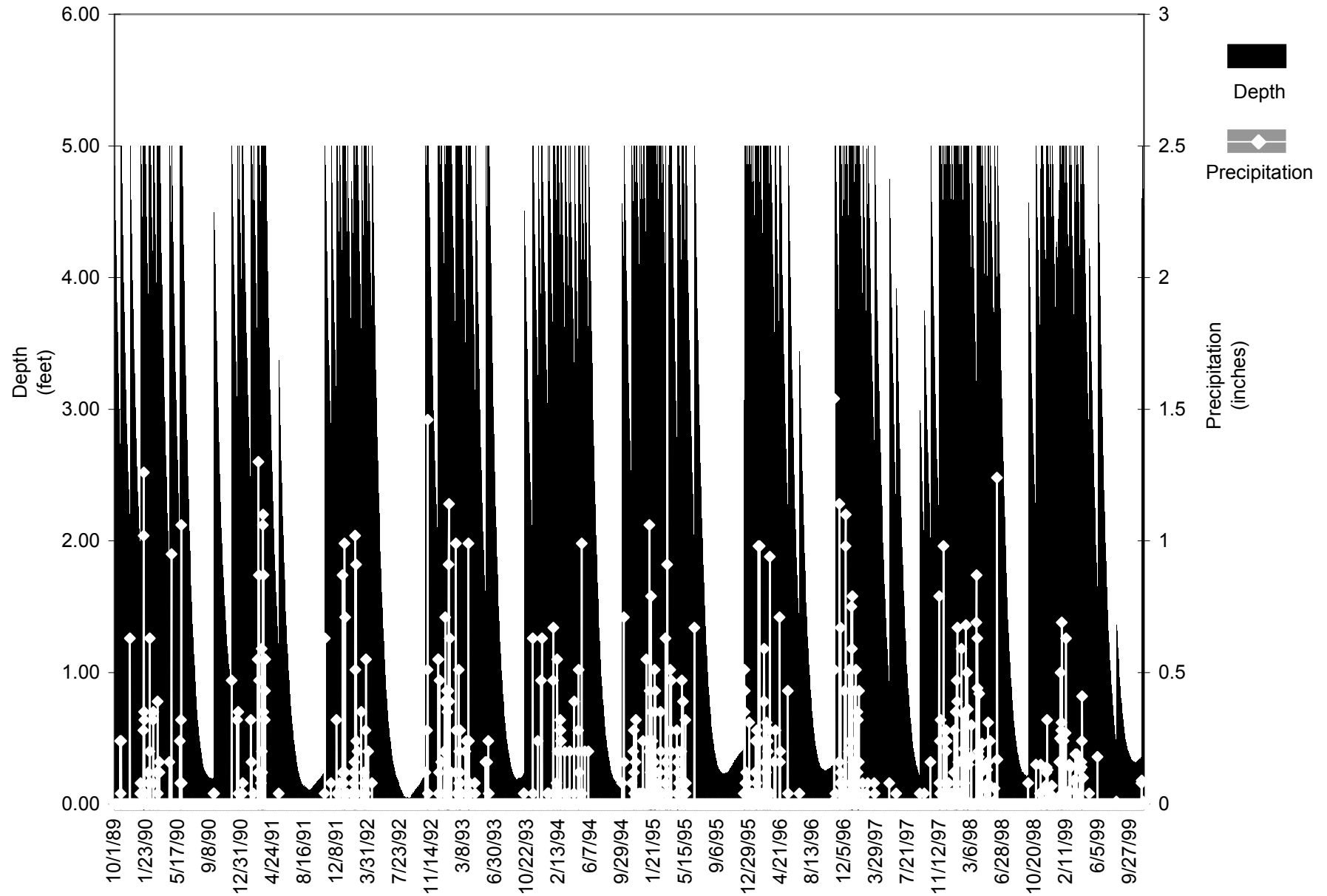
Figure 3-4 Model Results of Water Depth for Oxbow 1 Using Daily Fresno Station Data for Ten Years
